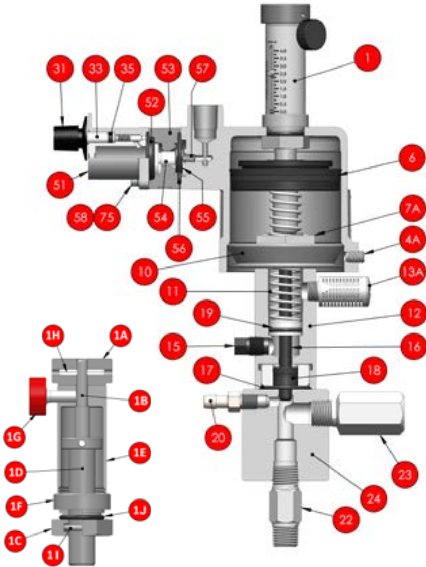
ITEM 1 ASSEMBLY
