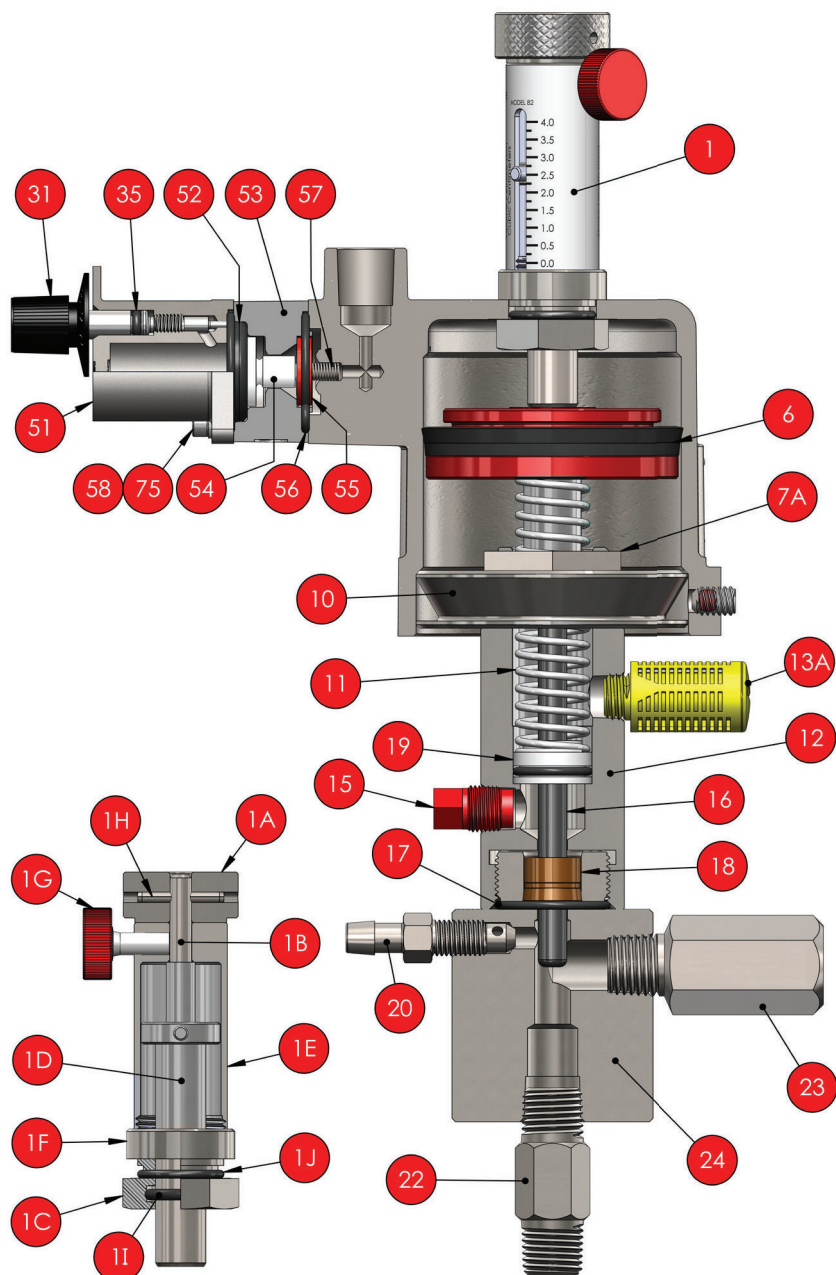
ITEM 1 ASSEMBLY
