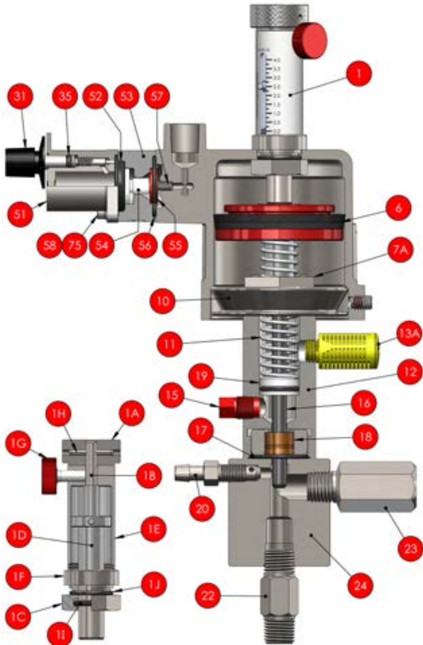
ITEM 1 ASSEMBLY
