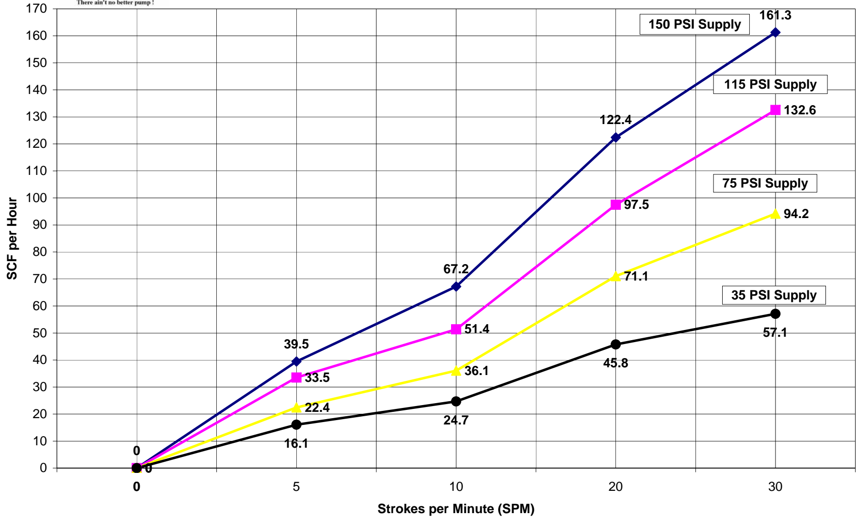
Model 44/64/84/164 Air/Gas Consumption Results obtained from controlled test conditions with instrument air Figures are approximate, actual results may vary depending on conditions
