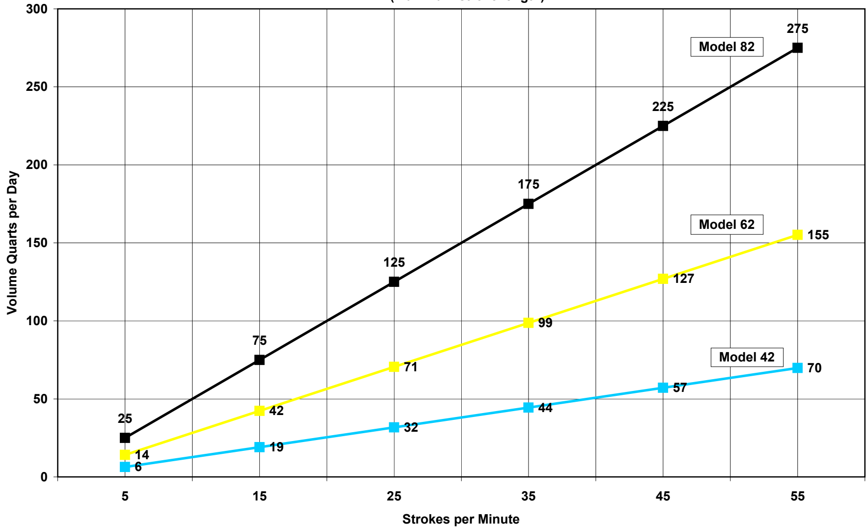
Model 42/62/82 Conversion Strokes per Minute to Quarts per Day Flow Rates are approximate-Pump Setting Guage should be used to insure accuracy (maximum stroke length)
